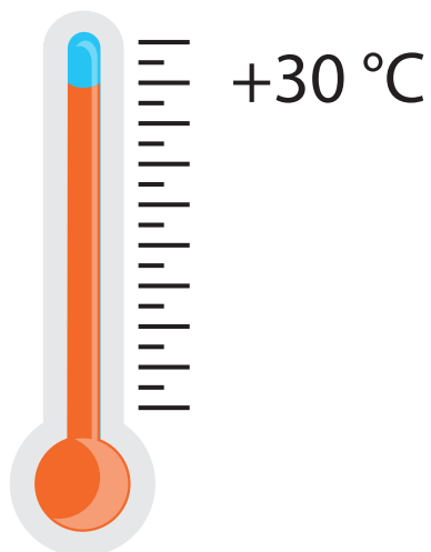
heat wave
