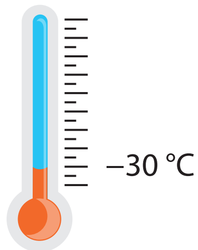
freezing
